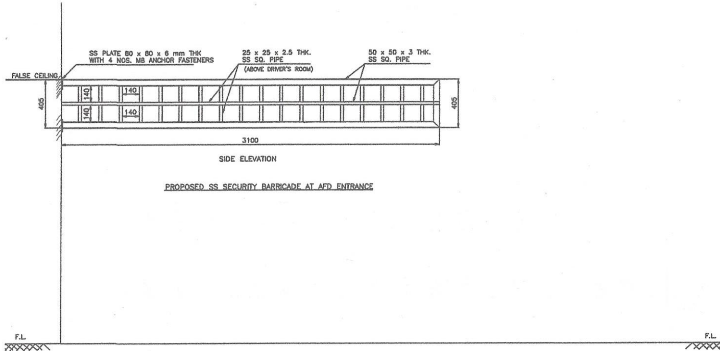
PROPOSED SS SECURITY BARRICADE AT AFD ENTRANCE
