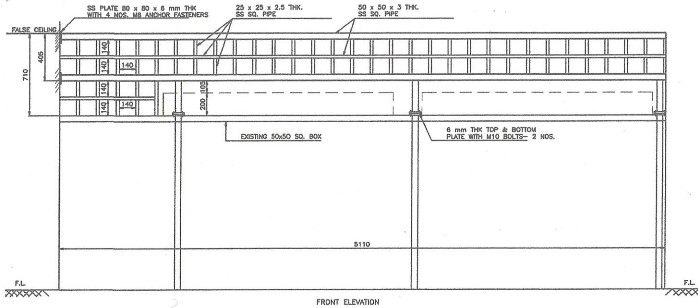
PROPOSED SS SECURITY BARRICADE AT AFD ENTRANCE
